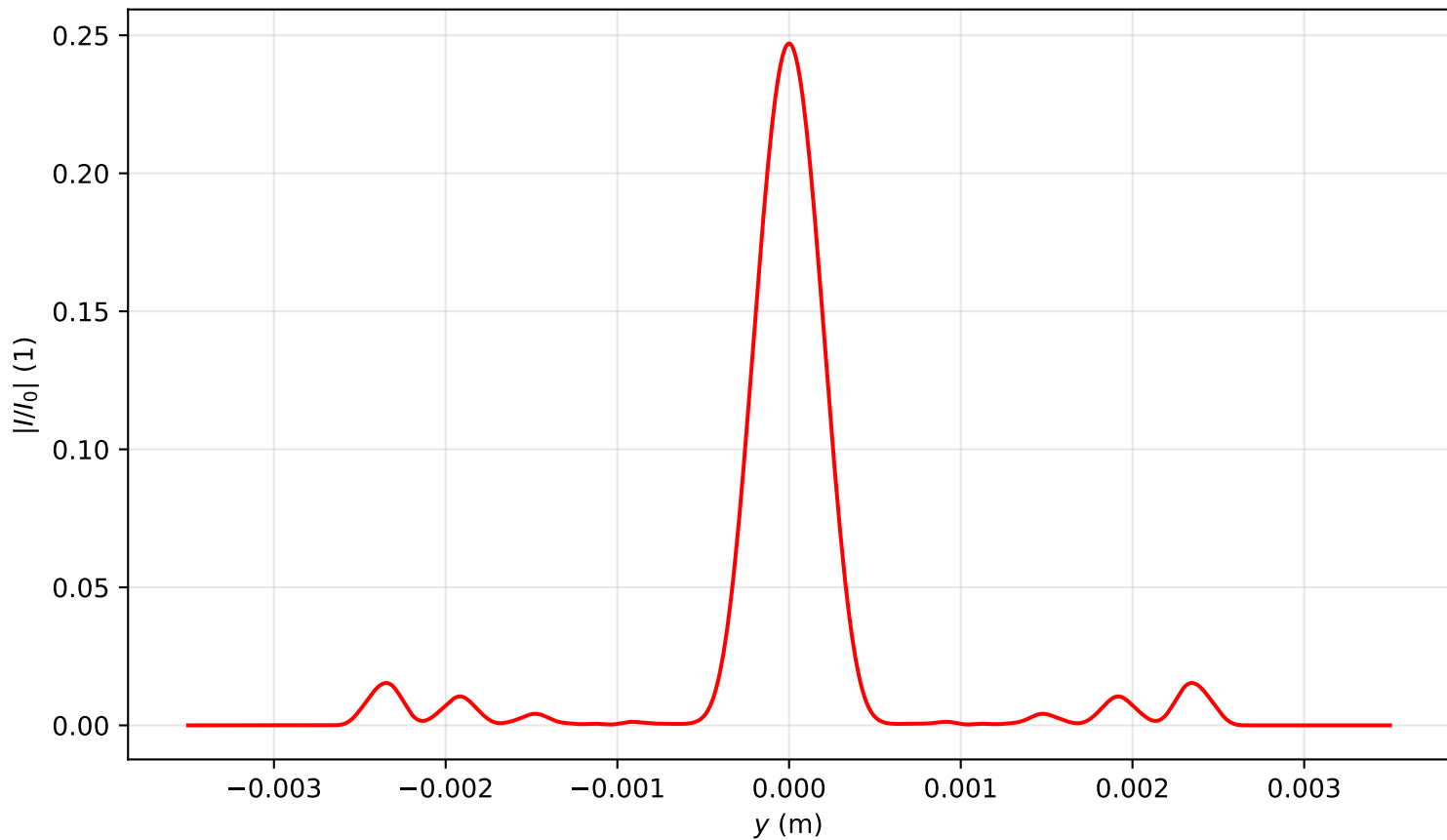
Intensity profile I(x=0, y, z=2.866)/I_0 , P_{in}=9.0P_{cr} , artificial time
